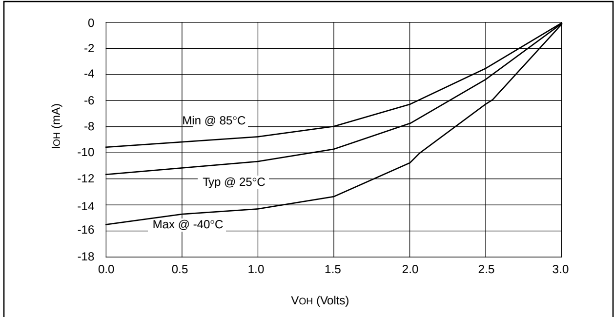
FIGURE 12-18: I_{OH} vs. V_{OH} , V_{DD} = 3V
