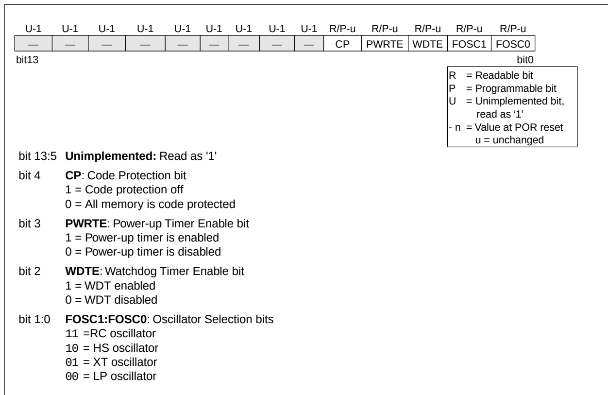
FIGURE 8-1: CONFIGURATION WORD
