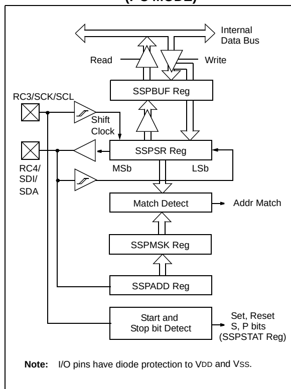
FIGURE 13-6: MSSP BLOCK DIAGRAM (I 2 C MODE)
