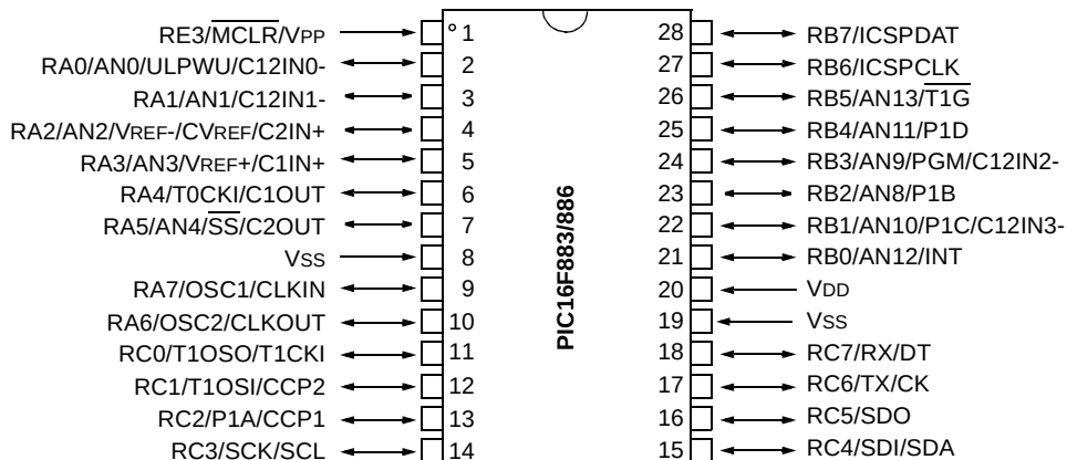
28-pin PDIP, SOIC, SSOP
