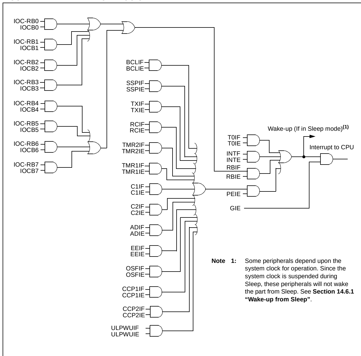
FIGURE 14-7: INTERRUPT LOGIC
