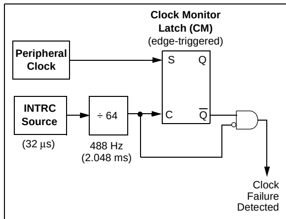
FIGURE 19-3: FSCM BLOCK DIAGRAM
