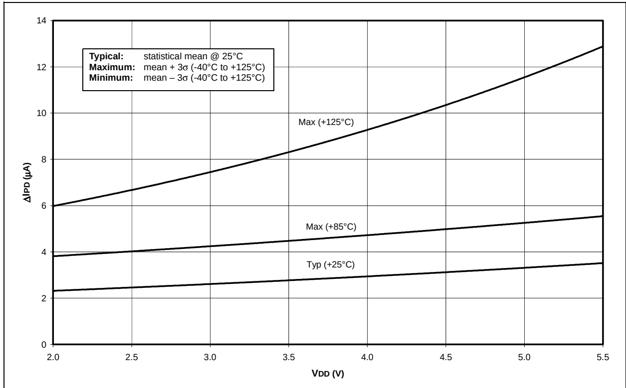
FIGURE 23-30: \Delta I_{PD} WDT, -40°C TO +125°C SLEEP MODE, ALL PERIPHERALS DISABLED
