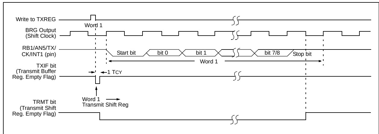
FIGURE 16-3: ASYNCHRONOUS TRANSMISSION
