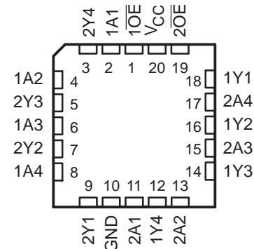
SN54LVT244 . . . FK PACKAGE (TOP VIEW)
