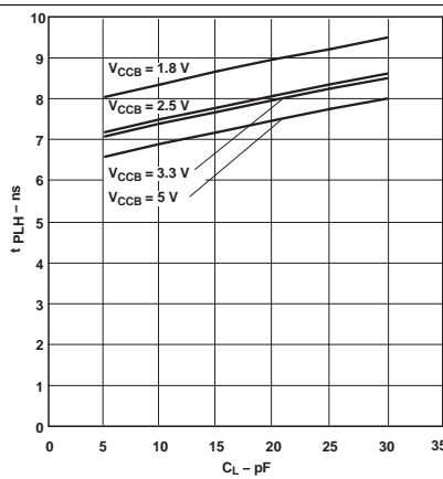
Figure 4. Typical Propagation Delay of Low-to-High (B to A) vs Load Capacitance T_A = 25^\circ\text{C} , V_{CCA} = 1.8\text{ V}
