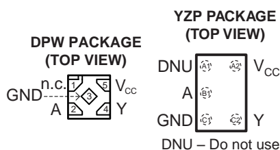
YZP Package Terminal Assignments
