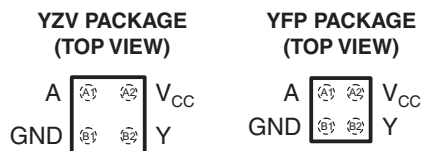
YZV and YFP Package Terminal Assignments
