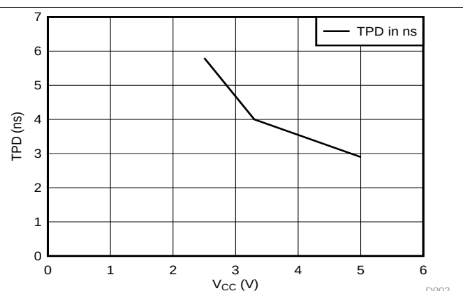
Figure 2. TPD vs V_{CC} at 25^\circ\text{C}
