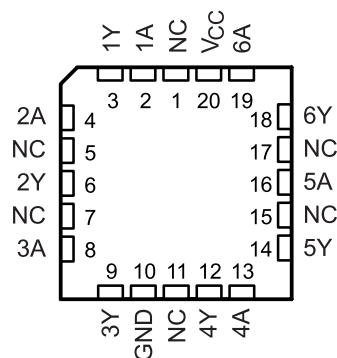
SN54LV06A . . . FK PACKAGE (TOP VIEW)
