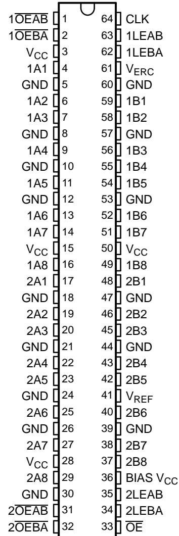
DGG PACKAGE (TOP VIEW)
