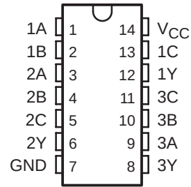
SN54ALS10A, SN54AS10 . . . J PACKAGE SN74ALS10A, SN74AS10 . . . D OR N PACKAGE (TOP VIEW)
