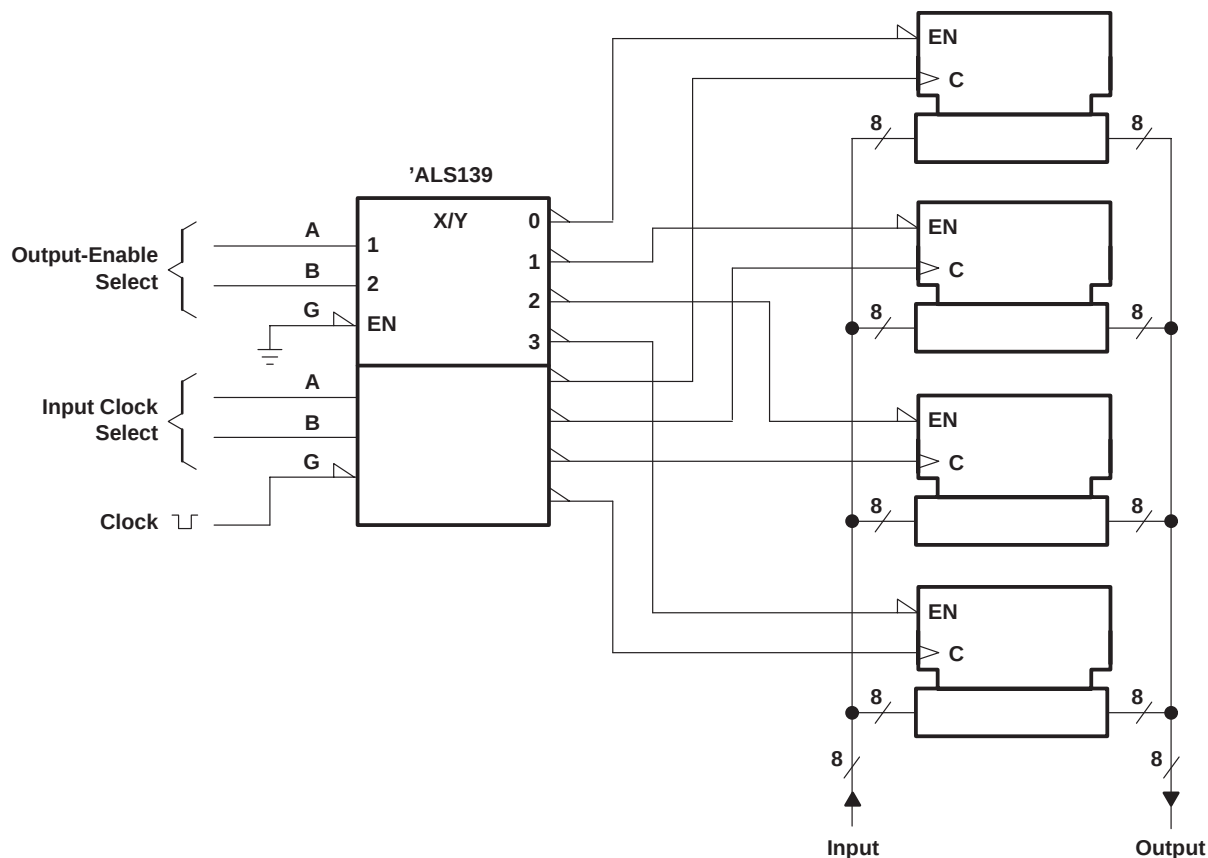
Figure 1. Expandable 4-Word by 8-Bit General File Register
