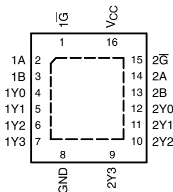
SN74AHC139 ... RGY PACKAGE (TOP VIEW)
