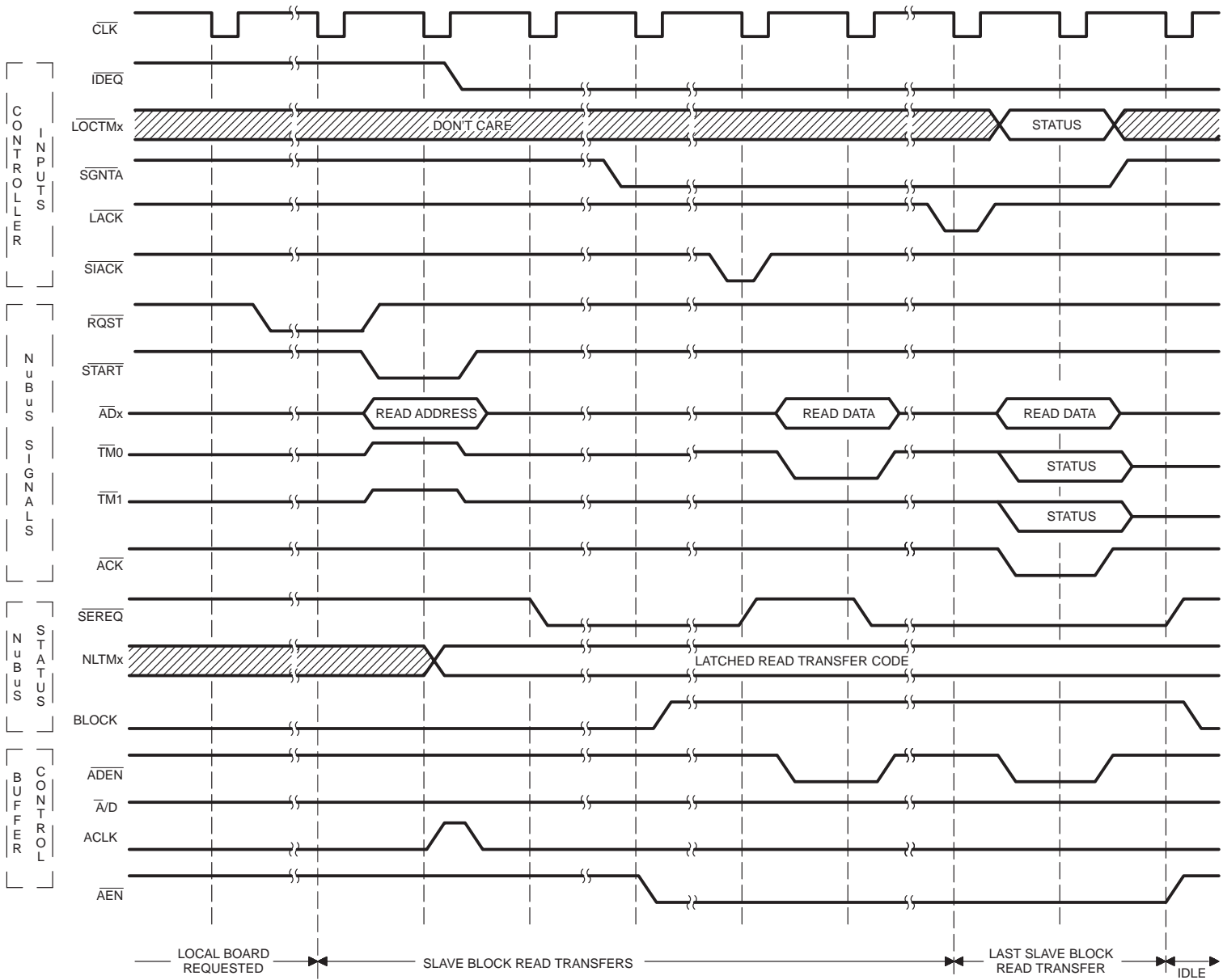
Figure 14. Slave Block-Read Transfer Cycle
