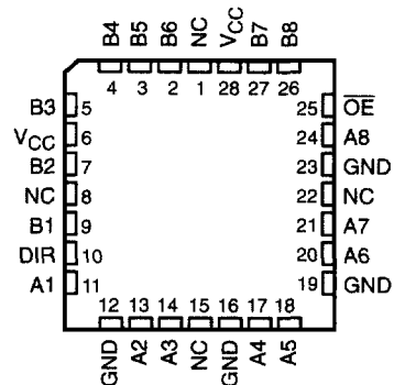
SN54ABTH25245 ... FK PACKAGE (TOP VIEW)
