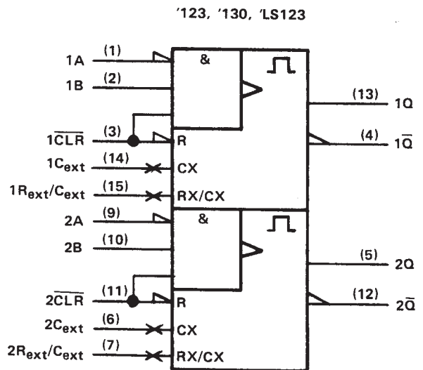
logic symbol†
