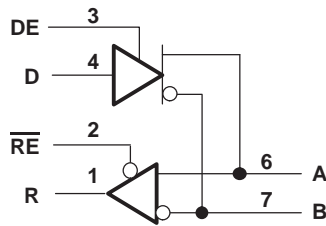
SN65MLVD200A, SN65MLVD204A
