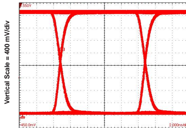
SN65MLVD200A RECEIVER OUTPUT EYE PATTERN 100 Mbps, 2^{15}-1 PRBS, C_L = 15 \text{ pF}
