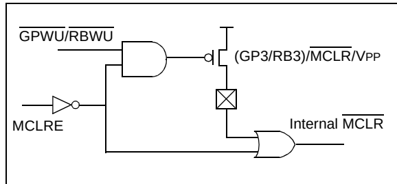
FIGURE 7-7: \overline{\text{MCLR}} SELECT
