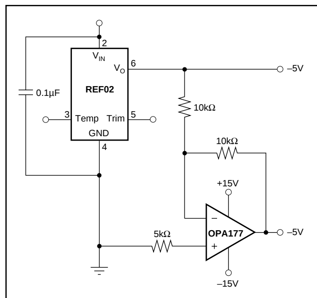
FIGURE 2. \pm 5\text{V} Precision Reference.
