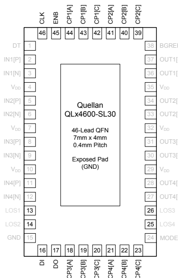
FIGURE 26. PIN DIAGRAM HIGHLIGHTING PINS USED FOR DYNAMIC CONTROL OF THE QLx4600-SL30
