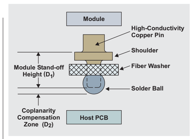
Figure 4. Detailed view of a Solderball Pin
