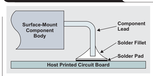
Figure 1. Acceptable SMT solder joint
