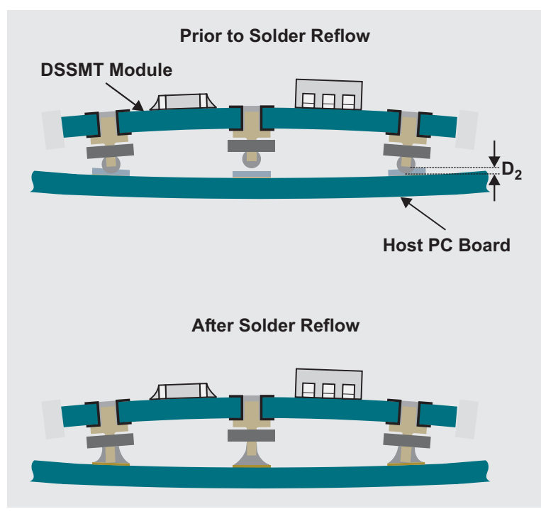
Figure 5. Behavior of DSSMT module during reflow
