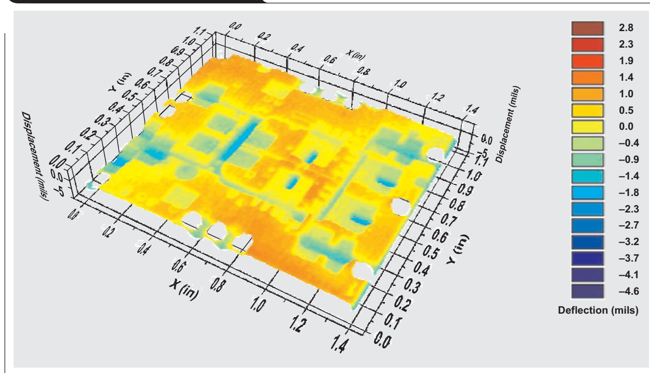
Figure 6. Shadow moiré 3D plot at 260°C
