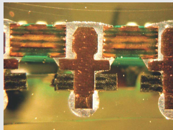
Figure 7. Cross section of pin/module solder joint
