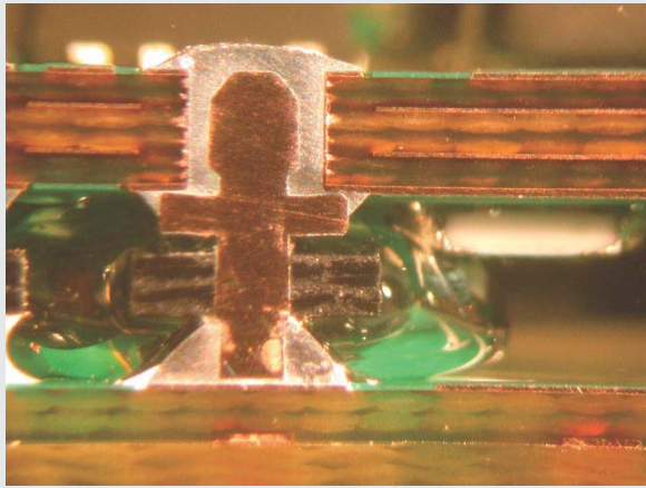
Figure 8. Cross section after reflow to host PCB
