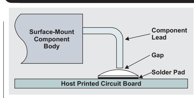
Figure 2. Excessive gap prevents fillet formation
