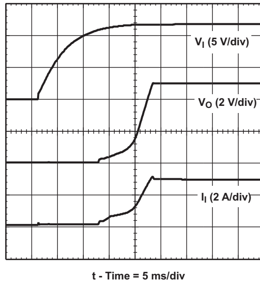
Figure 26. Power-Up Waveforms
