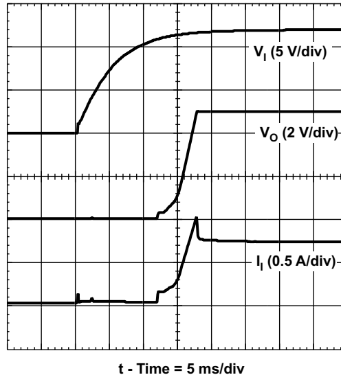
Figure 29. Power-Up Waveforms
