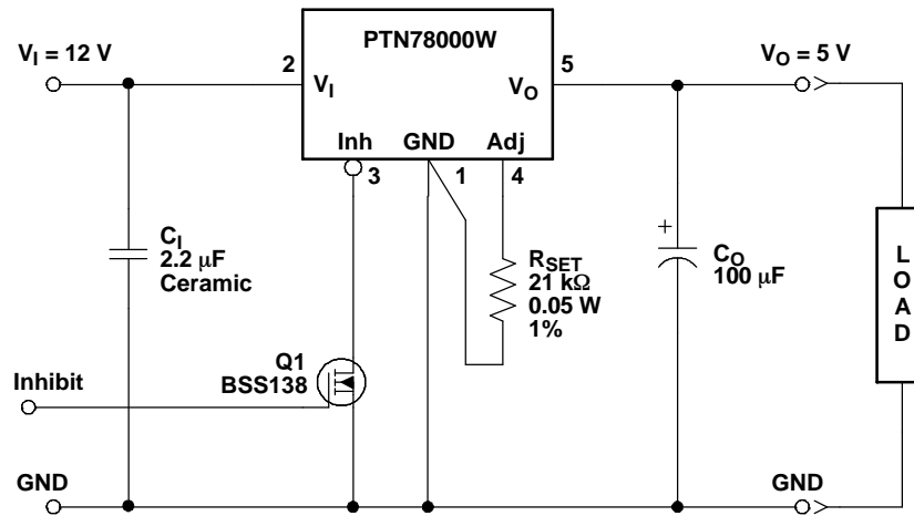
Figure 30. On/Off Inhibit Control Circuit
