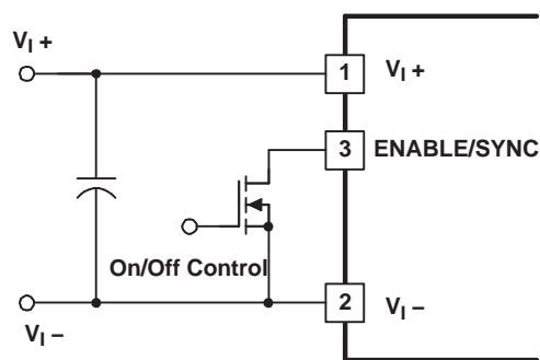
Figure 15. Typical On/Off Enable Control Circuit
