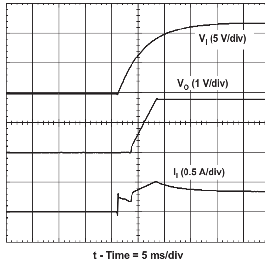
Figure 11. Power-Up Waveforms
