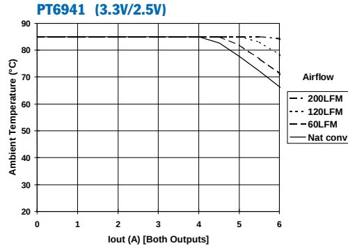
Safe Operating Area Curves; V_{in}=5V (See Note B)
