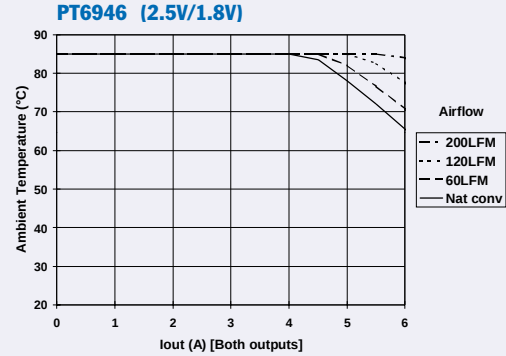
Safe Operating Area Curves; V_{in}=3.3V/5V (See Note B)
