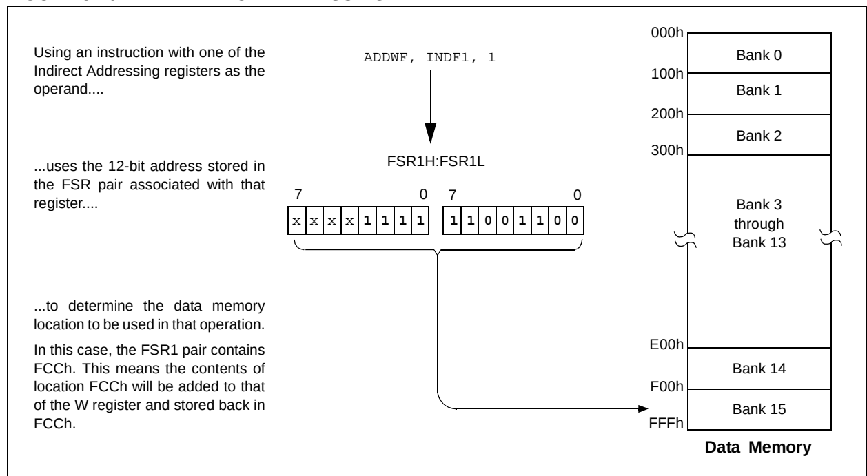
FIGURE 5-10: INDIRECT ADDRESSING
