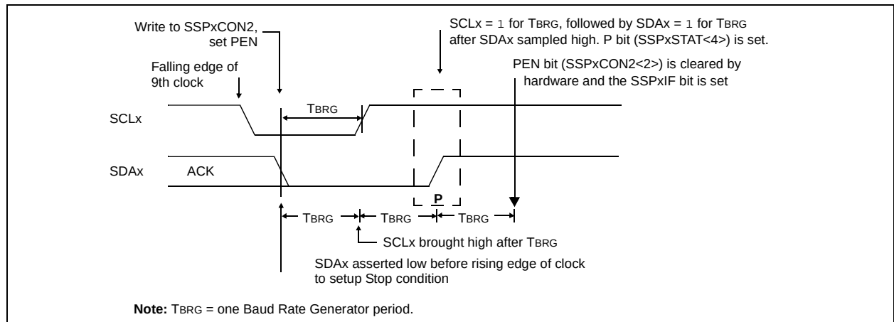
FIGURE 18-26: STOP CONDITION RECEIVE OR TRANSMIT MODE
