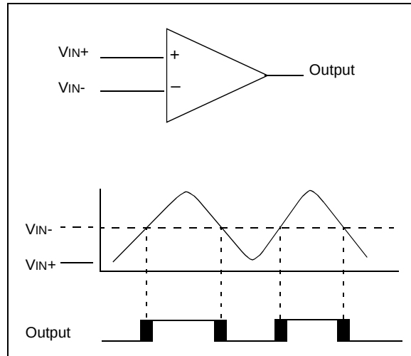
FIGURE 21-2: SINGLE COMPARATOR
