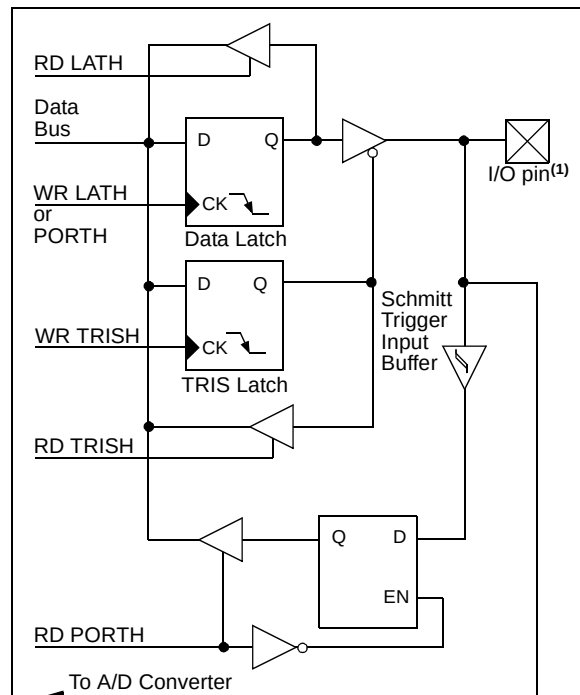
FIGURE 10-19: RH7:RH4 PINS BLOCK DIAGRAM IN I/O MODE
