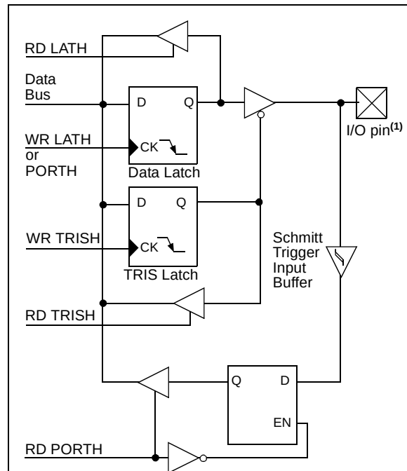
FIGURE 10-18: RH3:RH0 PINS BLOCK DIAGRAM IN I/O MODE
