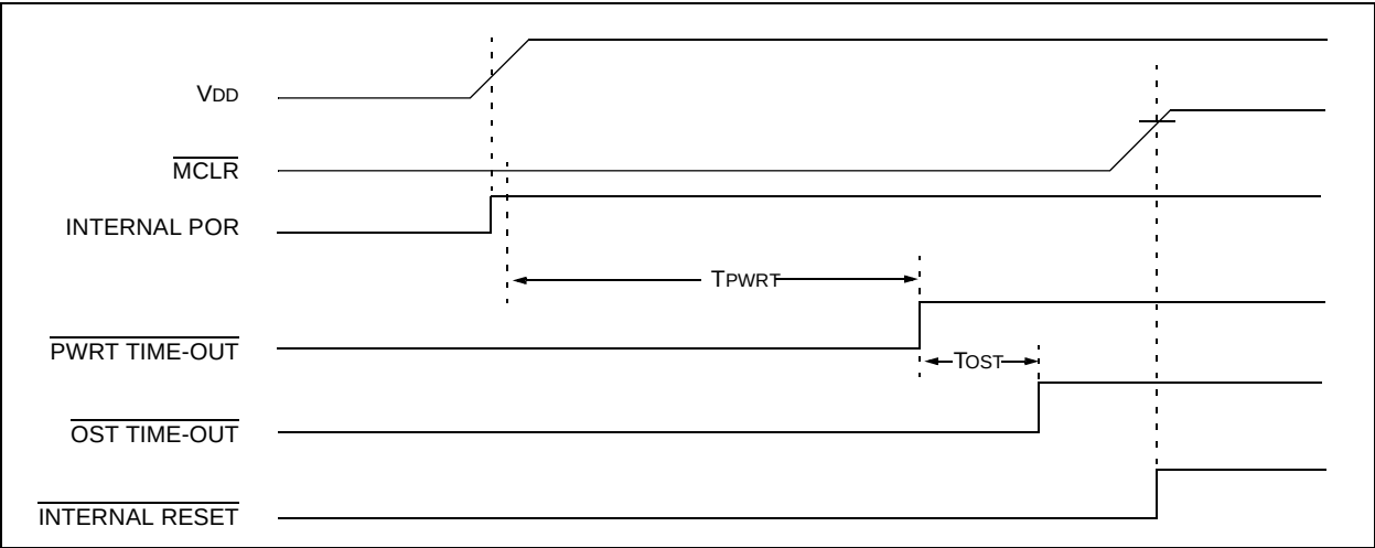
FIGURE 12-8: TIME-OUT SEQUENCE ON POWER-UP ( \overline{\text{MCLR}} NOT TIED TO \text{V}_{\text{DD}} ): CASE 2
