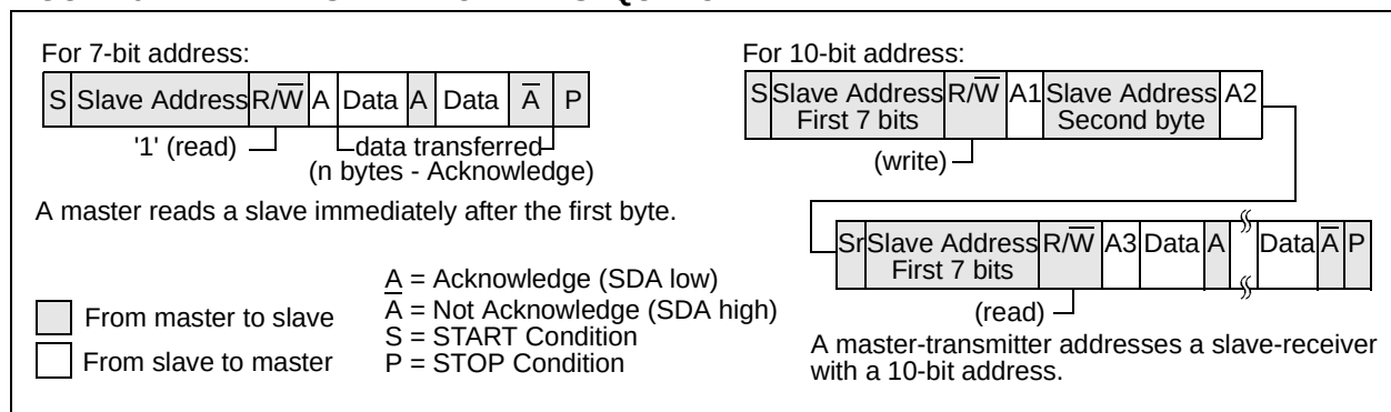
FIGURE 9-12: MASTER-RECEIVER SEQUENCE
