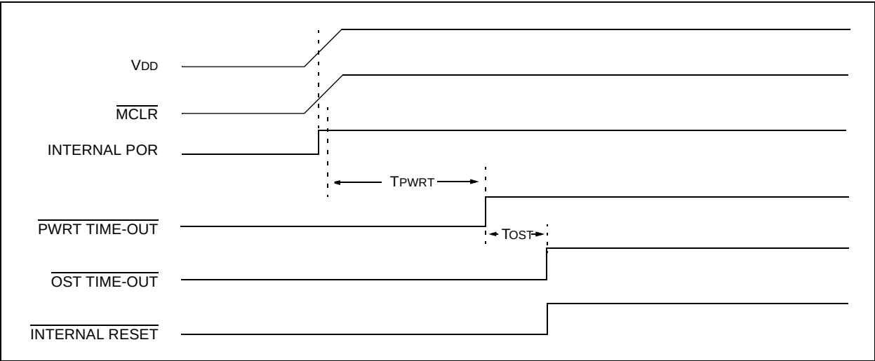
FIGURE 12-9: TIME-OUT SEQUENCE ON POWER-UP ( \overline{\text{MCLR}} TIED TO \text{V}_{\text{DD}} )
