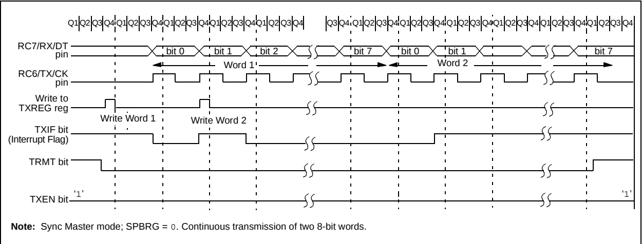
FIGURE 10-9: SYNCHRONOUS TRANSMISSION
