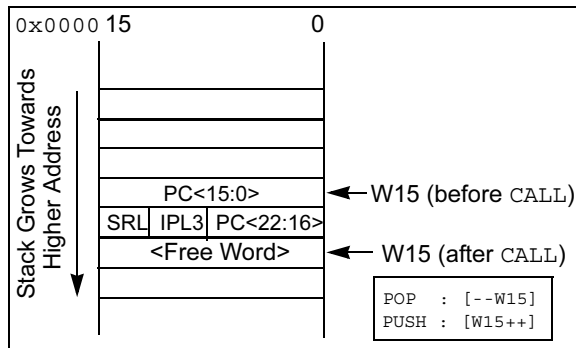
FIGURE 5-1: INTERRUPT STACK FRAME
