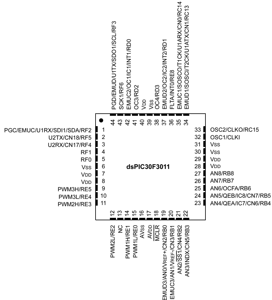
44-Pin QFN
