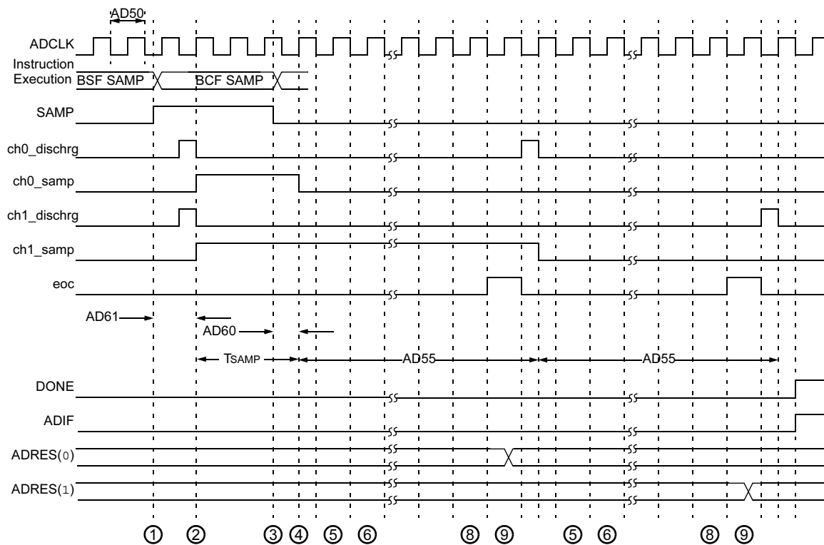
FIGURE 24-26: 10-BIT HIGH-SPEED A/D CONVERSION TIMING CHARACTERISTICS (CHPS = 01, SIMSAM = 0, ASAM = 0, SSRC = 000)
