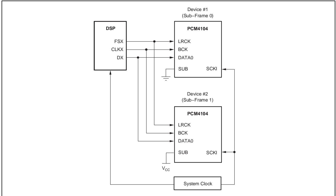
Figure 12. TDM Connection
