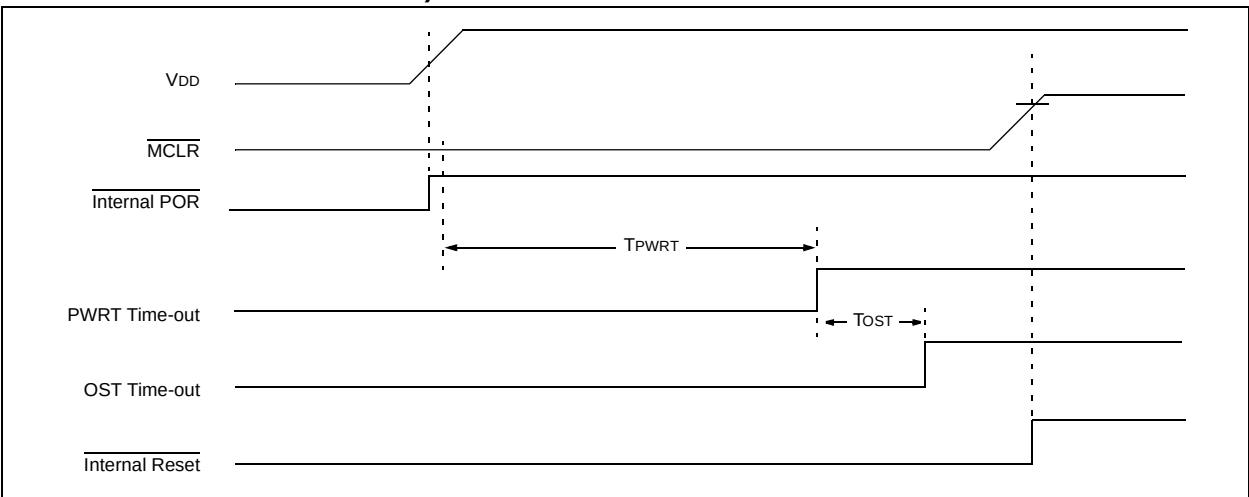
FIGURE 12-5: TIME-OUT SEQUENCE ON POWER-UP ( \overline{\text{MCLR}} TIED TO V_{\text{DD}} THROUGH RC NETWORK): CASE 2
