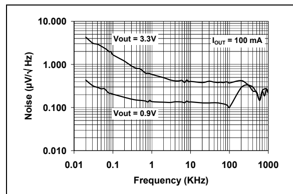
FIGURE 2-30: Output Noise
