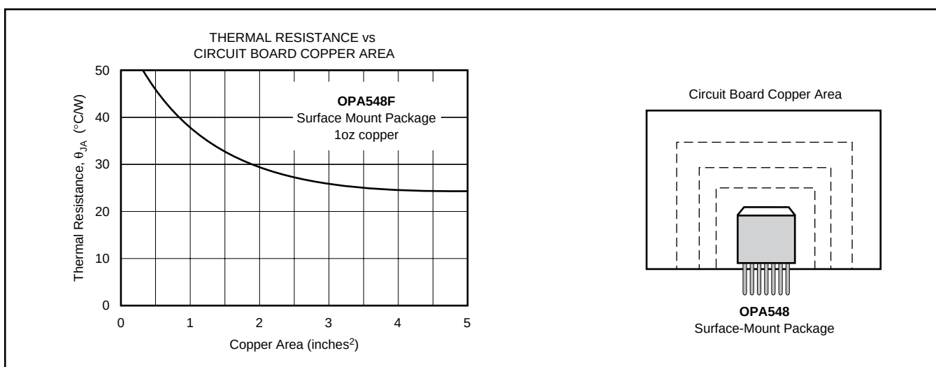
FIGURE 6. DDPK Thermal Resistance vs Circuit Board Copper Area.
