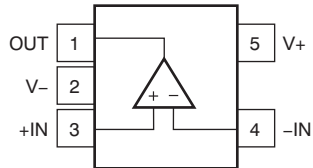
OPA376 SC70-5 (TOP VIEW)
