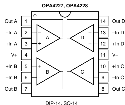
DIP-14, SO-14
