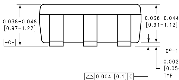
5-Pin SOT23-5 NS Package Number MF05A
