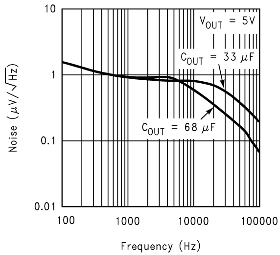
Output Noise Density, V_{OUT} = 5V
