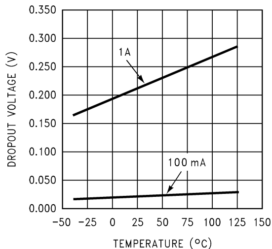
Drop-Out Voltage Vs Temperature ( I_L = 100mA , 1A , V_{OUT} = 2.5V , Dropout at 50mV Down)
