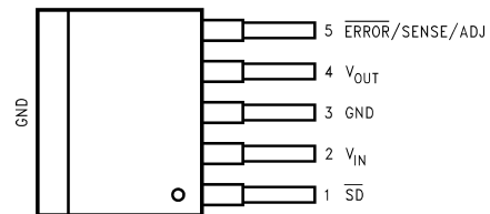
Top View TO263-5 Package
