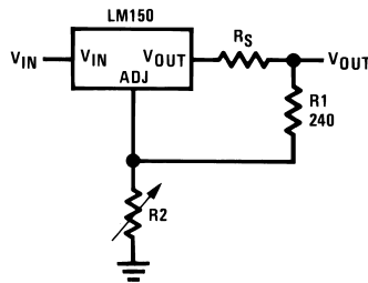
Figure 3. Regulator with Line Resistance in Output Lead
