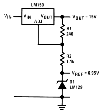
Figure 12. Regulator and Voltage Reference
