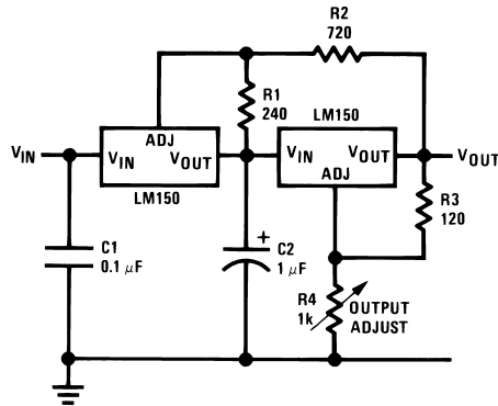
Figure 22. Tracking Preregulator
