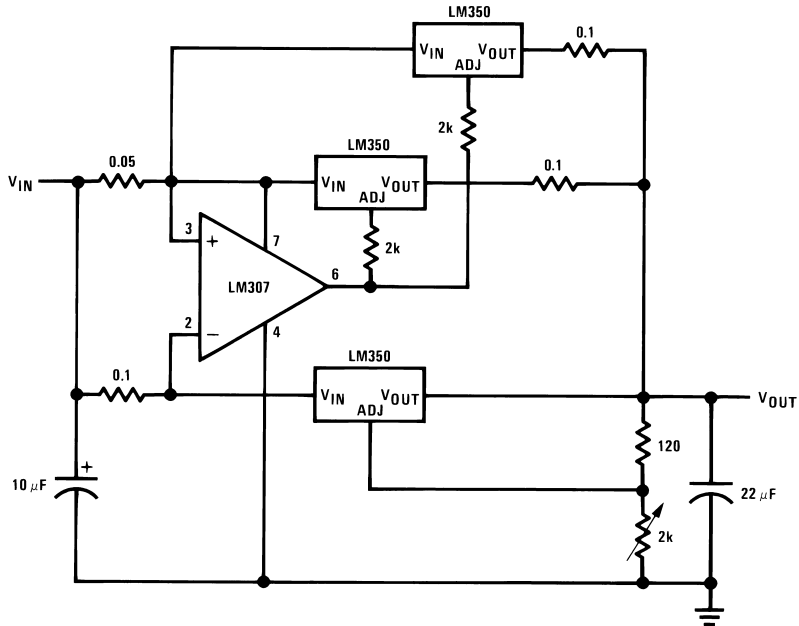
Figure 13. 10A Regulator
