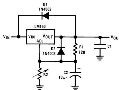
Figure 4. Regulator with Protection Diodes
