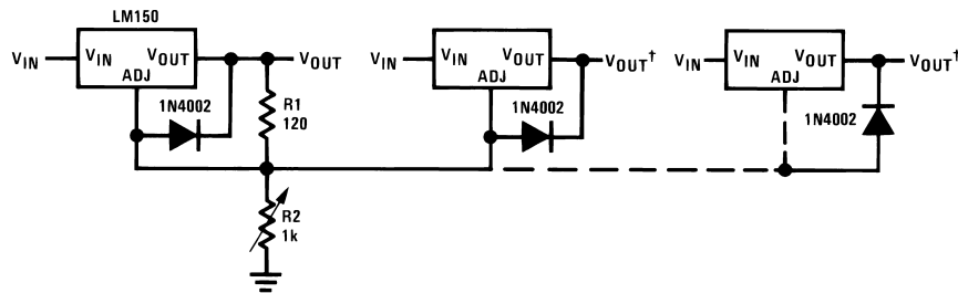
Figure 23. Adjusting Multiple On-Card Regulators with Single Control*
