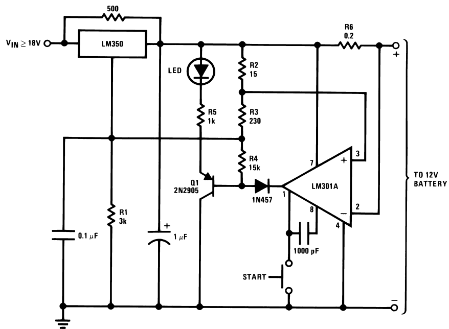
Figure 17. 12V Battery Charger
