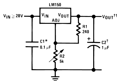
Figure 6. 1.2V–25V Adjustable Regulator
