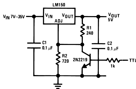
Figure 14. 5V Logic Regulator with Electronic Shutdown*
