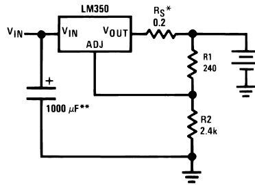
Figure 25. Simple 12V Battery Charger
