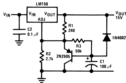
Figure 8. Slow Turn-ON 15V Regulator
