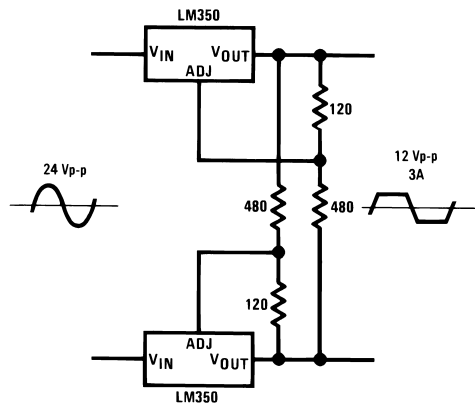
Figure 24. AC Voltage Regulator
