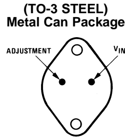
Figure 1. Bottom View
