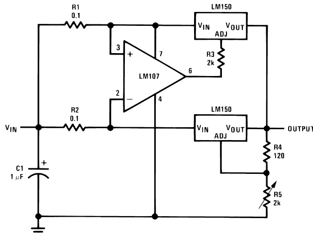
Figure 30. 6A Regulator
