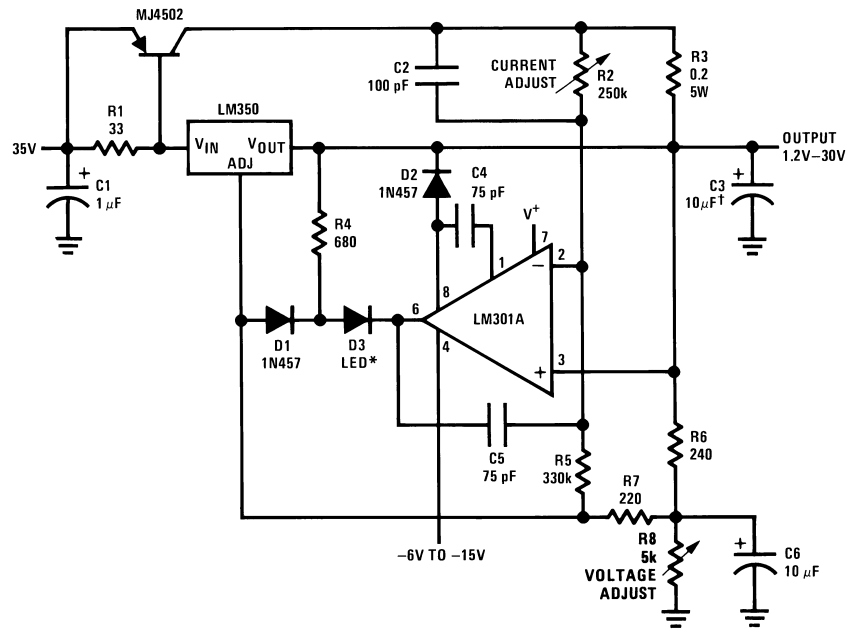
Figure 16. 5A Constant Voltage/Constant Current Regulator
