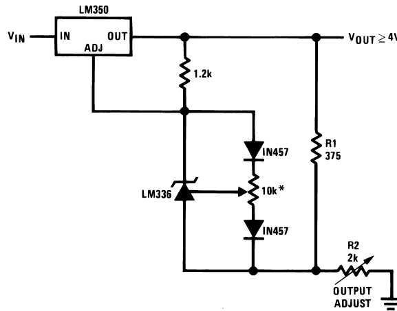
Figure 7. Precision Power Regulator with Low Temperature Coefficient
