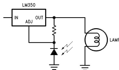
Figure 27. Light Controller
