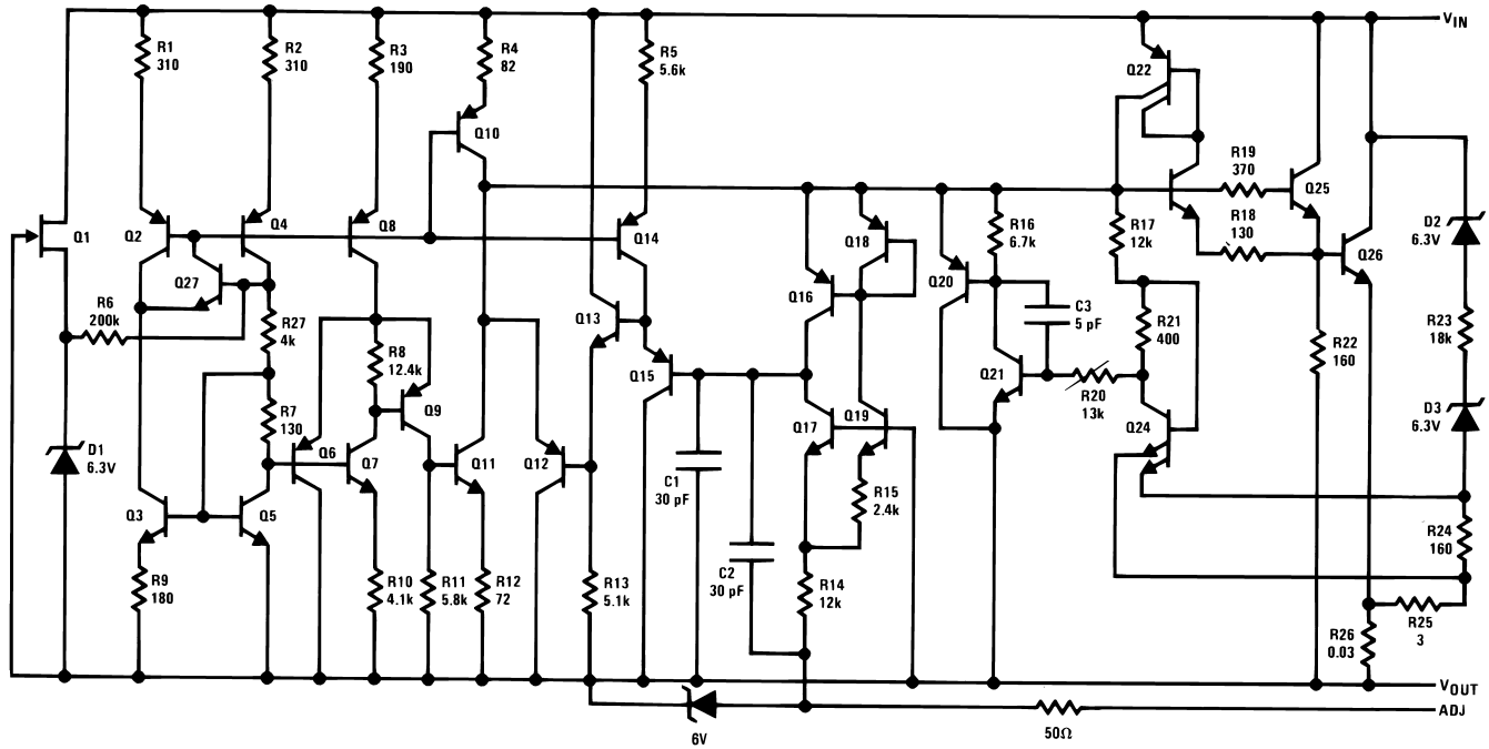
Figure 5. Schematic Diagram
