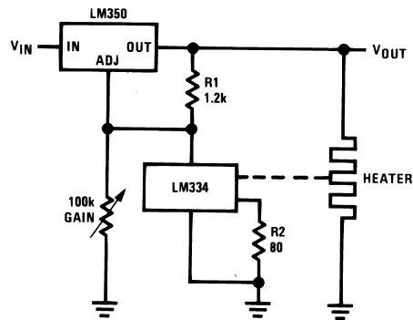
Figure 26. Temperature Controller
