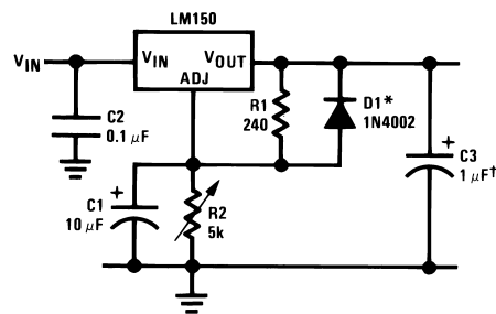
Figure 9. Adjustable Regulator with Improved Ripple Rejection
