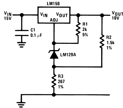
Figure 10. High Stability 10V Regulator
