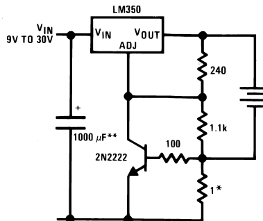
Figure 29. Current Limited 6V Charger
