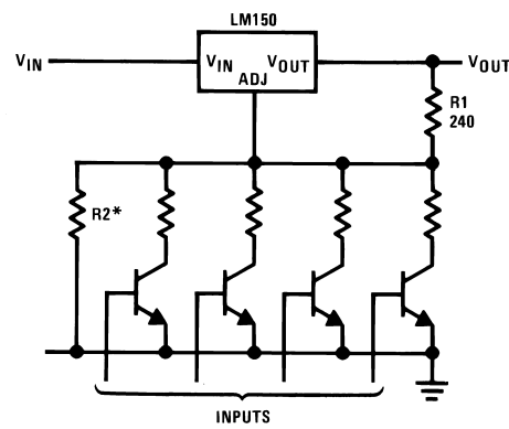
Figure 11. Digitally Selected Outputs
