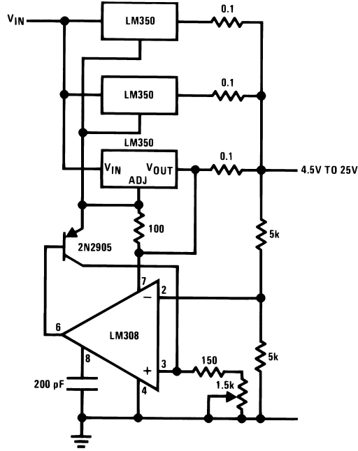
Figure 28. Adjustable 10A Regulator
