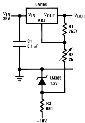
Figure 15. 0 to 30V Regulator
