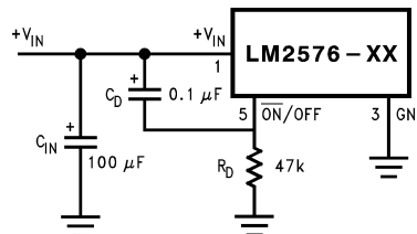
Figure 12. Delayed Startup
