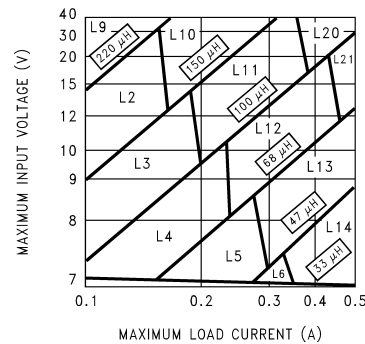
Figure 11. LM2671-5.0
