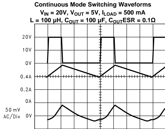
A: V_{SW} Pin Voltage, 10 V/div. B: Inductor Current, 0.2 A/div C: Output Ripple Voltage, 50 mV/div AC-Coupled
