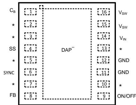
Figure 2. 16-Lead LLP Surface Mount Package Top View
