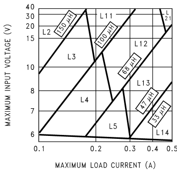
Figure 10. LM2671-3.3
