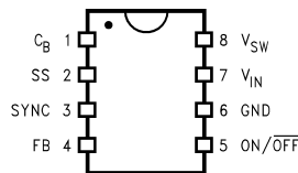
Figure 3. SO-8/DIP Package 8-Lead Package Top View
