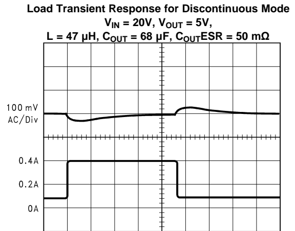
A: Output Voltage, 100 mV/div, AC-Coupled B: Load Current: 100 mA to 400 mA Load Pulse
