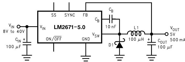
Figure 1. Fixed Output Voltage Versions
