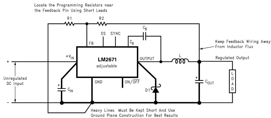
Figure 8. Standard Test Circuits and Layout Guides Fixed Output Voltage Versions
