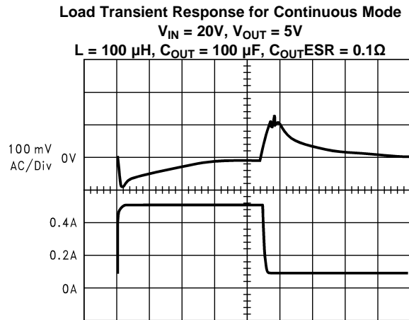
A: Output Voltage, 100 mV/div, AC-Coupled B: Load Current: 100 mA to 500 mA Load Pulse
