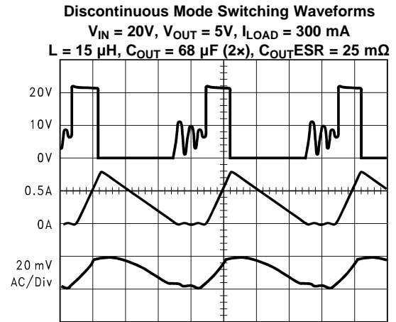
A: V_{SW} Pin Voltage, 10 V/div. B: Inductor Current, 0.5 A/div C: Output Ripple Voltage, 20 mV/div AC-Coupled
