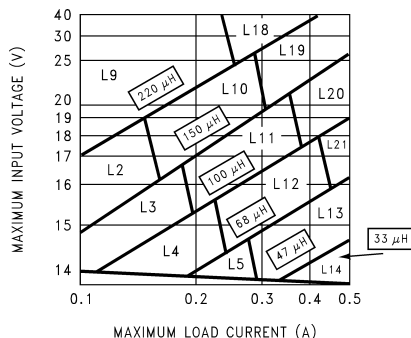
Figure 12. LM2671-12
