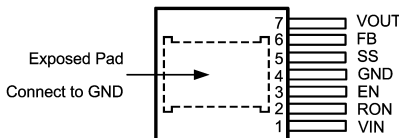
Figure 5. Top View - 7-Lead TO-PMOD
