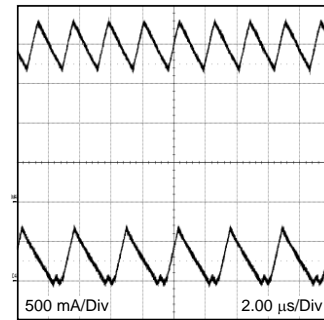
Figure 6. CCM and DCM Operating Modes V_{IN} = 12V , V_O = 3.3V , I_O = 2A/0.26A 2 \mu\text{sec/div}
