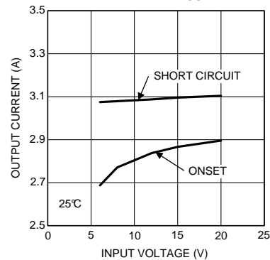
Current Limit 3.3V OUT @ 25°C
