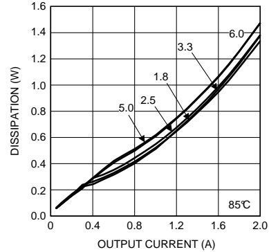
Dissipation 20V Input @ 85°C
