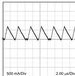
Figure 7. Transition Mode Operation V_{IN} = 12V , V_O = 3.3V , I_O = 0.29A 2 \mu\text{sec/div}
