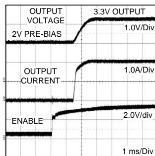
Figure 8. Pre-Biased Startup
