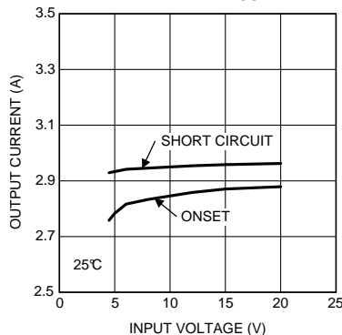
Current Limit 1.8V OUT @ 25°C
