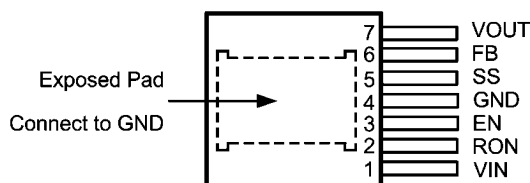
Top View 7-Lead TO-PMOD
