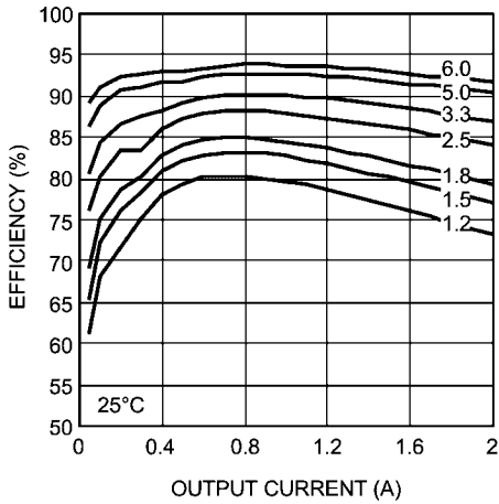
Efficiency 12V Input @ 25°C
