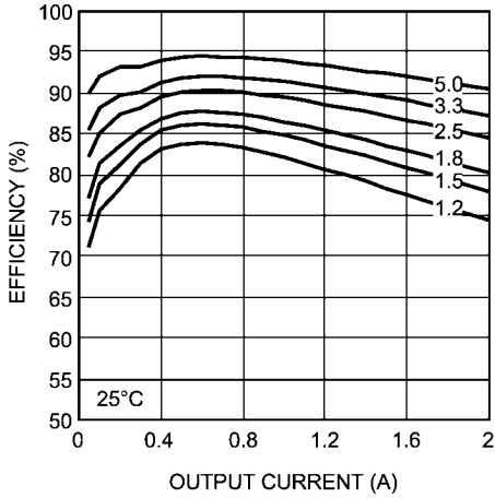
Efficiency 8V Input @ 25°C
