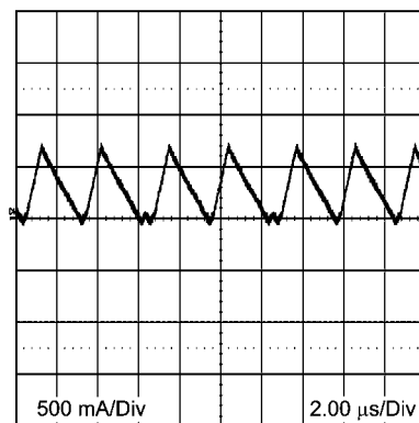
Transition Mode Operation V_{IN} = 12V, V_O = 3.3V, I_O = 0.29A \quad 2 \mu\text{sec/div}
