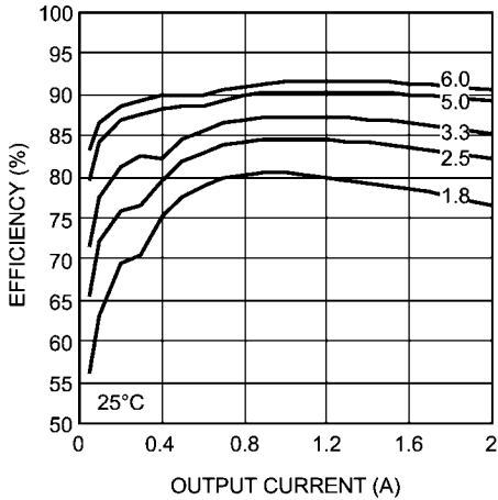
Efficiency 20V Input @ 25°C
