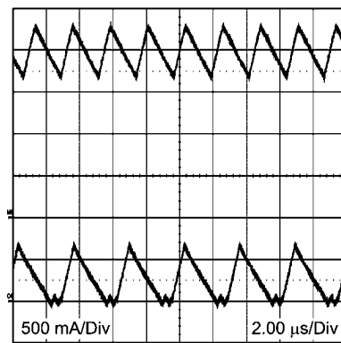
CCM and DCM Operating Modes V_{IN} = 12V, V_O = 3.3V, I_O = 2A/0.26A \quad 2 \mu\text{sec/div}
