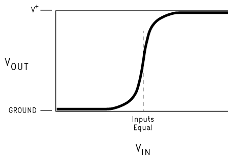
Figure 7. Without Positive Feedback (No Hysteresis)
