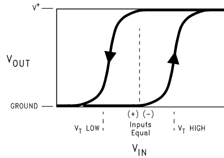
Figure 8. With Positive Feedback (Hysteresis or Memory)
