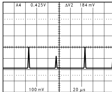
Figure 5. Measurement of the Shoot-Through Current
