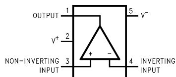
Figure 2. Top View
