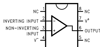
Figure 1. Top View
