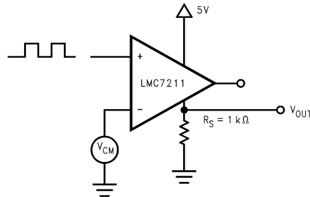
Figure 4. Circuit for Measurement of the Shoot-Through Current
