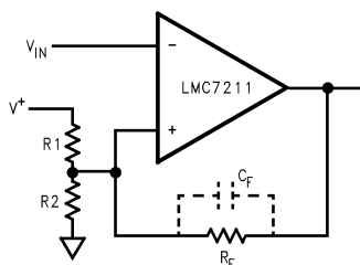
Figure 6. Positive Feedback for Hysteresis
