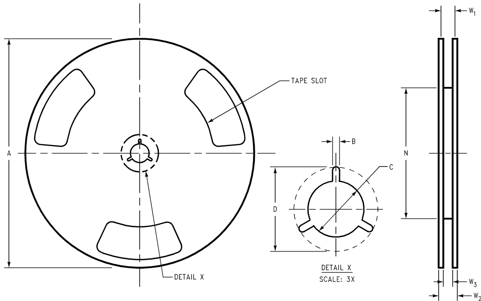
Figure 10. REEL DIMENSIONS
