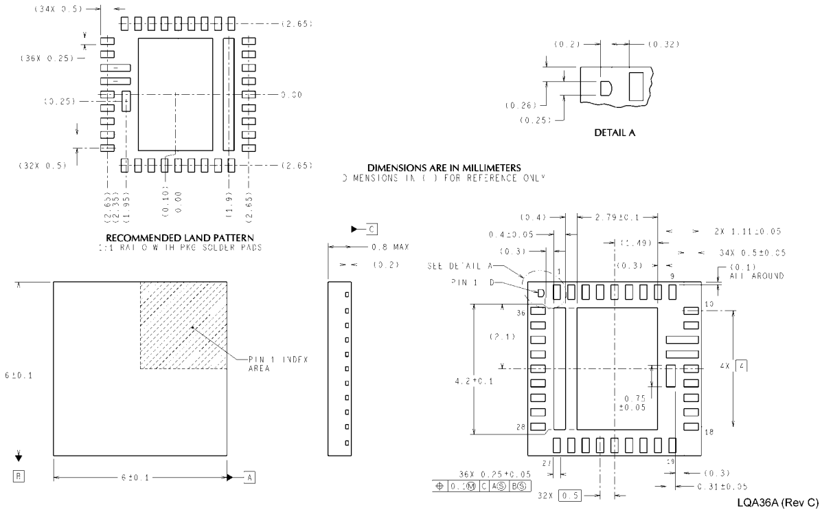
Leadless Leadframe Package (NS Package Number LQA036A), (Bottom View)
