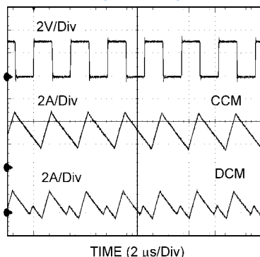
CCM and DCM Operating Modes V_{IN} = 12\text{V} , V_O = 3.3\text{V} , I_O = 3\text{A}/0.3\text{A}
