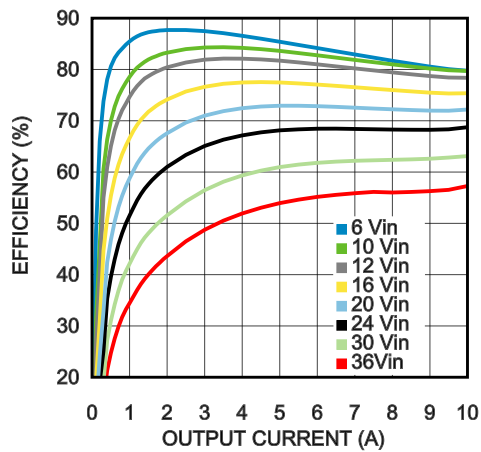
Efficiency 1.5V output @ 25°C
