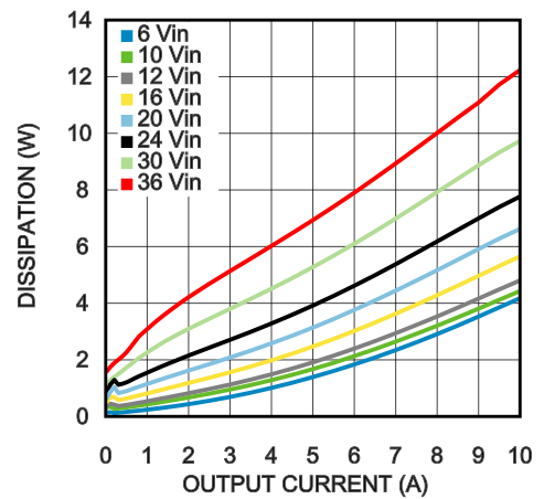
Dissipation 1.0V output @ 85°C
