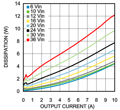
Dissipation 1.5V output @ 85°C
