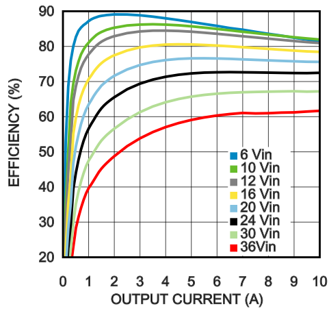
Efficiency 1.8V output @ 25°C
