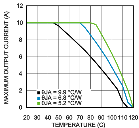
Thermal derating V_{IN} = 24V , V_{OUT} = 5.0V
