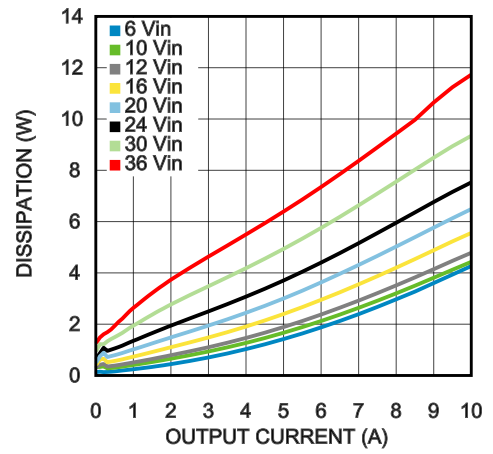
Dissipation 1.2V output @ 85°C
