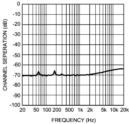
Crosstalk vs Frequency V_{DD} = 5.0V , V_{IN} = 1V_{P-P} , R_L = 32\Omega Mode 8, 80kHz BW
