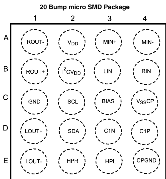
Top View (Bump Side Down) Order Number LM49200TL, LM49200TLX See NS Package Number TLA20BBA
