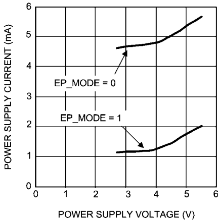
Supply Current vs Supply Voltage No Load, Mode 12 (2 plots, output gain amps on/off)
