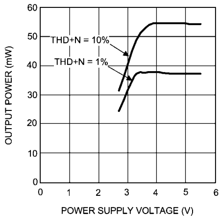
Output Power vs Supply Voltage f = 1kHz , R_L = 32\Omega SE Mode 8, 80kHz BW
