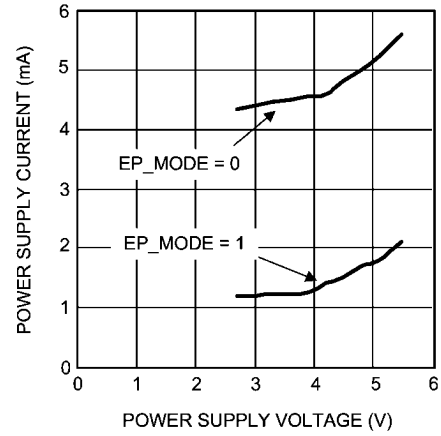
Supply Current vs Supply Voltage No Load, Mode 3 (2 plots, output gain amps on/off)
