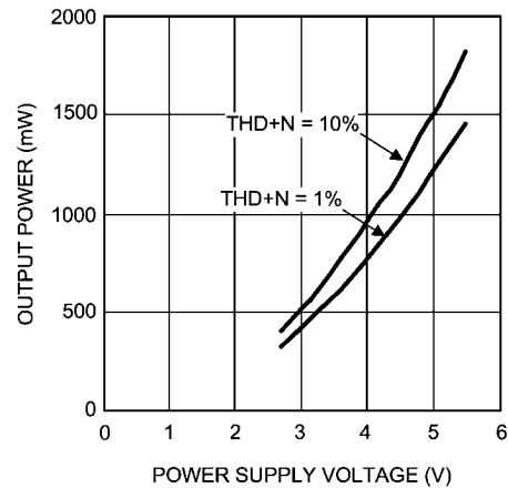
Output Power vs Supply Voltage f = 1kHz , R_L = 8\Omega BTL Mode 2, 80kHz BW
