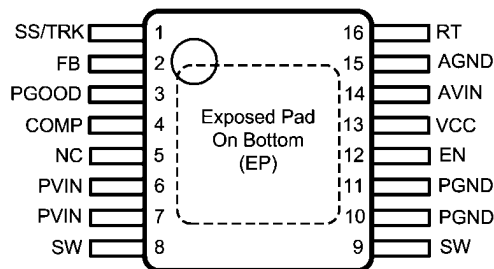
Top View eTSSOP-16 Package
