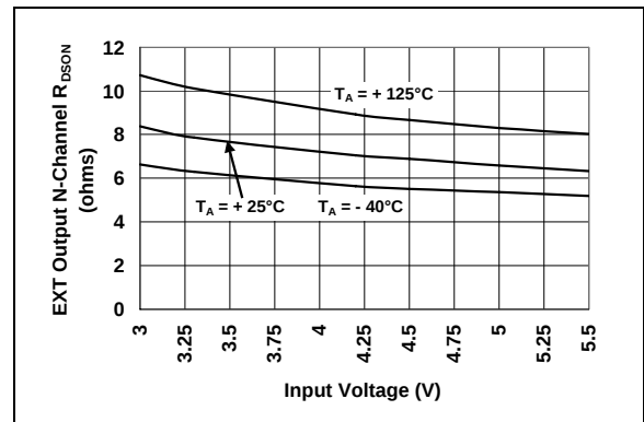
FIGURE 2-12: EXT Output N-channel R_{DS(on)} vs. Input Voltage.
