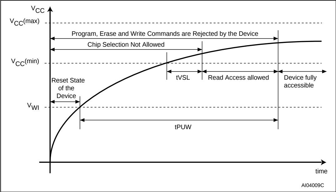
Figure 21. Power-up timing
