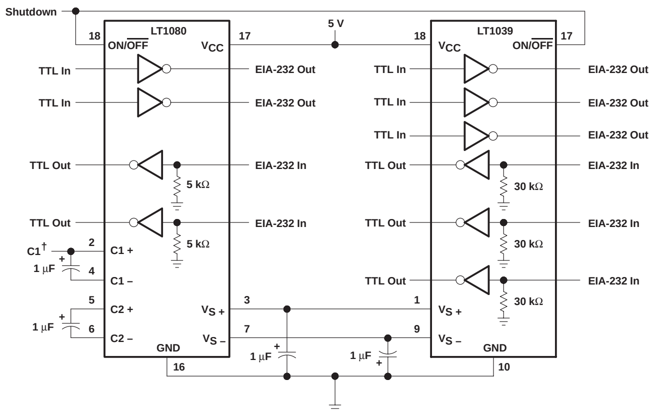
Figure 20. Powering External Circuitry
